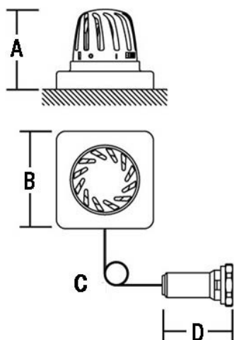
B1701 Liquid head with remote adjuster
