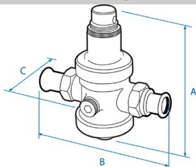
PS4PRV Pressure reducing valve
