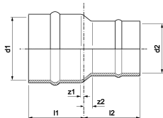
YP1R Coupling
