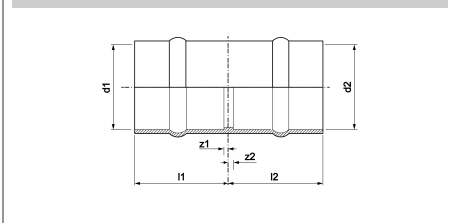
YP1 Coupling
